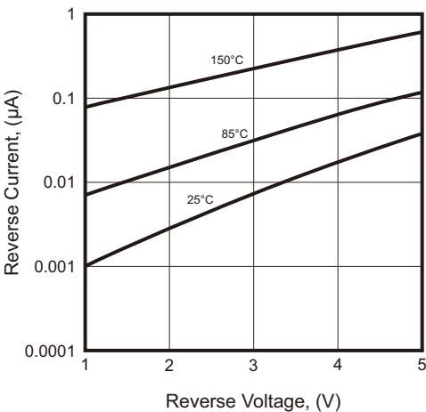
Fig.4 - Reverse Characteristics
